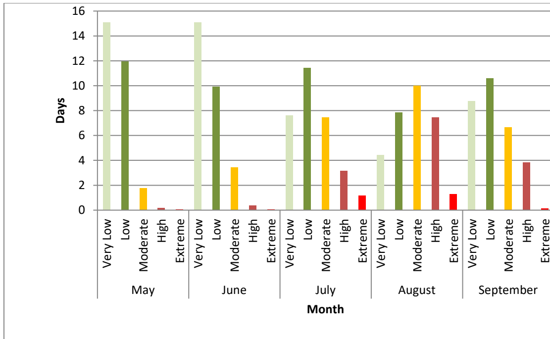
Figure 1. Average Fire Danger Class days per month (May to September) over 25 years in RDCK Area F recorded at the Smallwood weather station.
